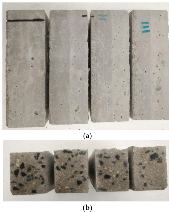
Figure 9. Section view of specimens and details of the layer boundaries (5, 10, 15, and 20 min from left to right). (a) side view—visible boundaries; (b) section view.
