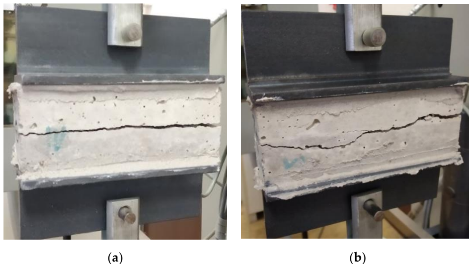
Figure 11. Specimen crack patterns: (a) regular failure on the layer interface areas and (b) an irregular crack.
